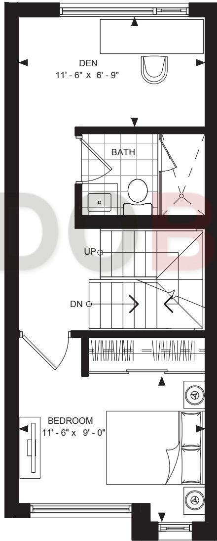
THIRD FLOOR
