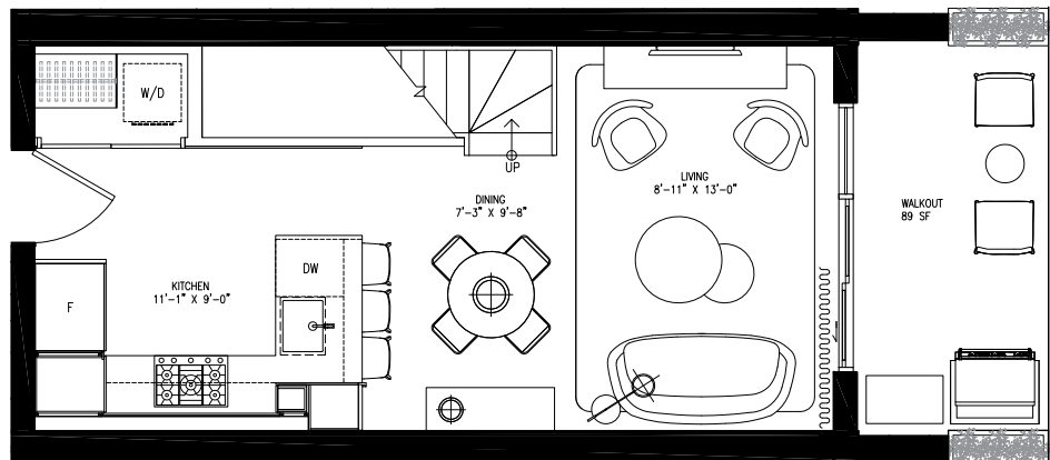
LIVING LEVEL
