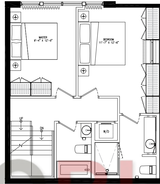
BEDROOM LEVEL
