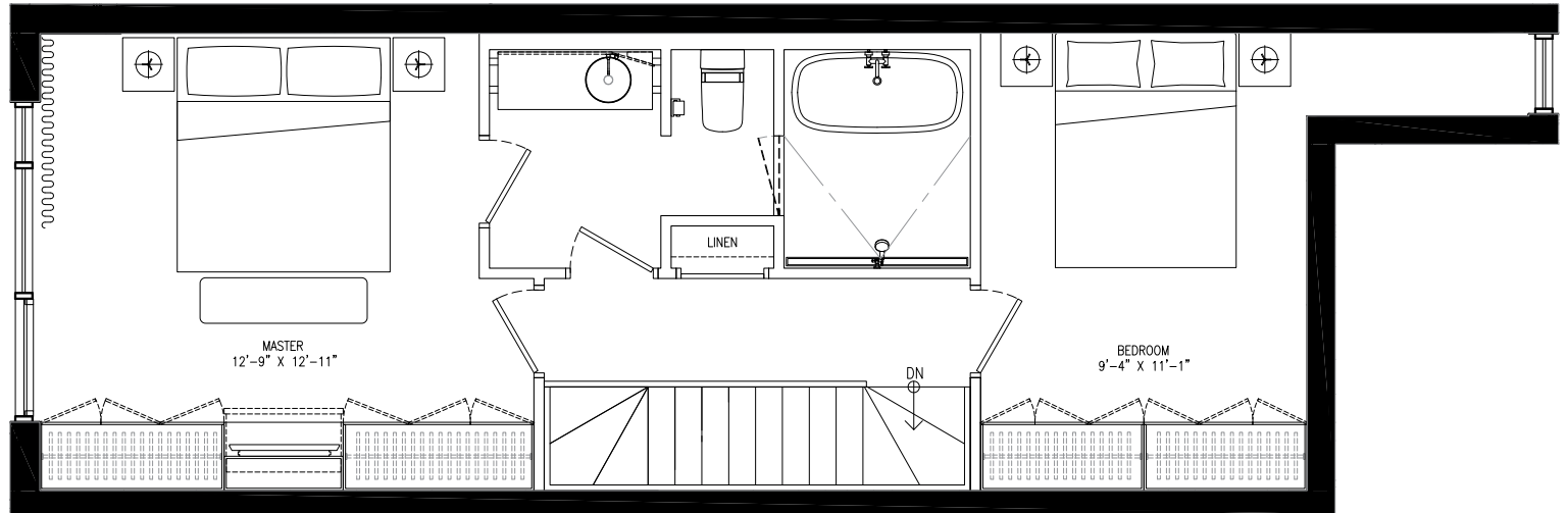
BEDROOM LEVEL
