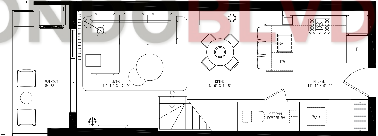
LIVING LEVEL
